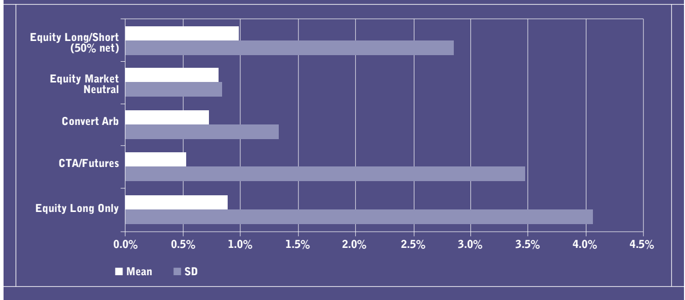
Figure 2: Comparison of Risk
