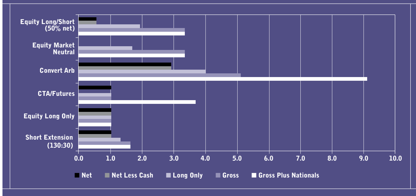
Figure 1: Summary of Leverage Ratios
